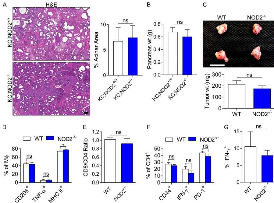
Figure 4. NOD2 deletion is not protective against PDA. (A and B) Cohorts of KC and KC;NOD2 -/- mice were sacrificed at 6 mo of life. Mean n = 6/group. (A) Representative H&E-stained sections are shown, and the fraction of preserved acinar area was calculated ( P = NS). Bar, 200 \mu m. (B) Pancreas weights (wt) were recorded ( P = NS). (C–G) WT and NOD2 -/- mice were orthotopically implanted with KPC-derived tumor cells. (C) Mice were sacrificed at 21 d. Representative gross pictures of tumors and mean tumor weights are shown ( P = NS). n = 5/group. Bar, 1 cm. (D) Expression of CD206, TNF, and MHC II in TAMs were determined by flow cytometry. *, P < 0.05. M \Phi , macrophage. (E–G) Similarly, the intratumoral CD8 + /CD4 + T cell ratio ( P = NS); E), CD4 + T cell expression of CD44, IFN- \gamma , and PD-1 (F), and CD8 + T cell expression of IFN- \gamma (G) were assessed ( P = NS). Orthotopic tumor experiments in NOD2 -/- mice were repeated four times with similar results, and littermate controls were used. Unpaired Student's t test was used for statistical analyses.
