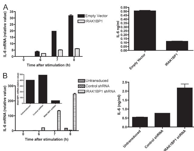
Figure 3. IRAK1BP1 inhibits LTA-stimulated IL-6 production.
