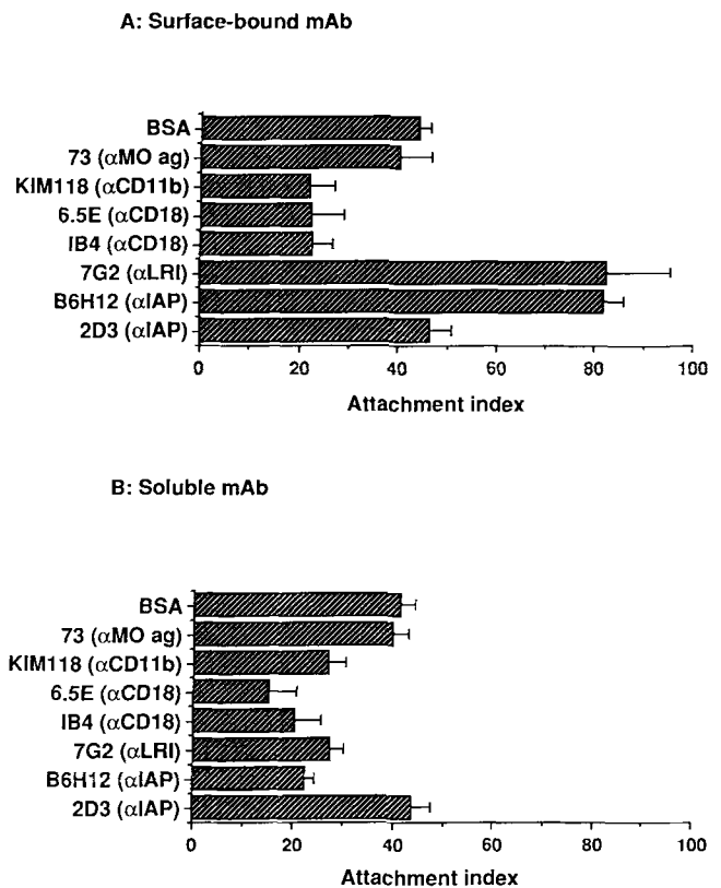
Figure 1. Effects of surface-bound (A) and soluble (B) mAbs on B. pertussis BP536 binding to human peripheral monocytes. Attachment index corresponds to the total number of bacteria adherent to 100 monocytes. Shown are mean values and standard errors, based on at least three experiments, each performed in triplicate.
