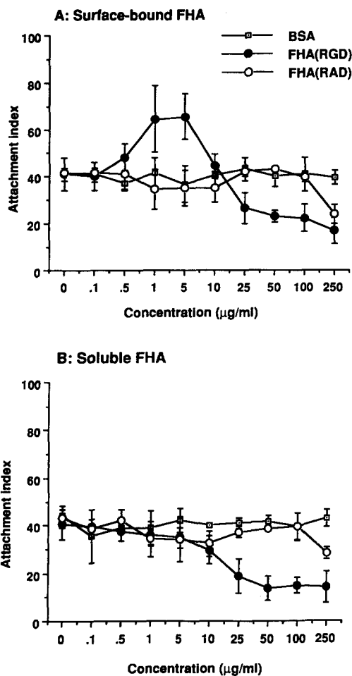
Figure 3. Effects of surface-bound (A) and soluble (B) FHA on BP536 binding to human peripheral monocytes. Wild-type RGD-containing FHA and mutant RAD-containing FHA are compared with BSA. The concentration of protein solutions used to precoat wells is indicated on the abscissa. Shown are mean values and standard errors, based on at least three experiments, each performed in triplicate.
