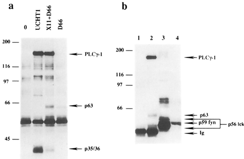
Figure 5. p63 coimmunoprecipitates with PLC \gamma -1 and is distinct from a tyrosine phosphorylated form of p56 lck or p59 lyn kinases. (a) Jurkat cells ( 10^7 for each point) were unstimulated (-), or activated with the CD3 mAb UCHT1 for 1 min, the CD2 mAb pair X11+D66 or the mAb D66 alone for 5 min. Cells were then lysed in a lysis buffer containing 1% digitonin and precleared lysates were immunoprecipitated with anti-PLC \gamma -1 mAb. Immune complexes were resolved by SDS-PAGE on a 8% acrylamide gel, and Western blot analysis using antiphosphotyrosine mAb 4G10 was performed. Positions of coimmunoprecipitating PLC \gamma -1, p35/36, and p63 are indicated. No bands except mAb H chains could be detected in immunoprecipitates performed with an irrelevant mAb (not shown). (b) In a separate experiment, Jurkat cells were left unstimulated (lane 1) or were activated using the CD2 mAb pair X11+D66 (lanes 2, 3, and 4), and treated as above. Lysates were then immunoprecipitated with anti-PLC \gamma -1 mAb (lanes 1 and 2) or rabbit antiserum recognizing the COOH-terminal residues of p56 lck (lane 3) or rabbit antiserum specific for p59 lyn (lane 4). Immunoprecipitates were resolved by SDS-PAGE and revealed using antiphosphotyrosine mAb 4G10. Positions of tyrosine phosphorylated bands of p56 lck , p59 lyn , and p63 are indicated.
