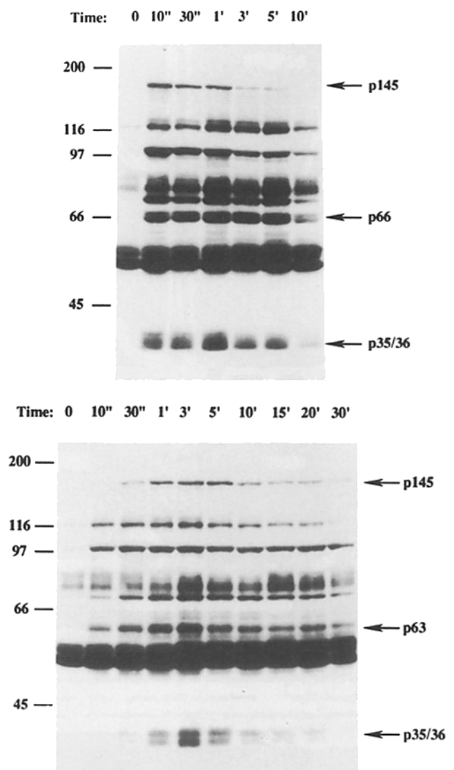
Figure 1. Different patterns of tyrosine phosphorylated proteins are induced after CD3 or CD2 stimulation. Jurkat cells ( 5 \times 10^6 ) were stimulated with the CD3 mAb UCHT1 (top) or with the CD2 mAbs X11+D66 (bottom) for the indicated times. Total cell extracts were resolved on a 8% polyacrylamide gel, transferred to nitrocellulose, and immunoblotted with antiphosphotyrosine mAb 4G10. Positions of molecular size markers are indicated. Exposition times were 10 s for each membrane. Parallel blotting using anti-PLC \gamma -1 mAb revealed no change in the amount of PLC \gamma -1 for each stimulation time, indicating that the same quantity of cellular extract was loaded for each sample (not shown).
