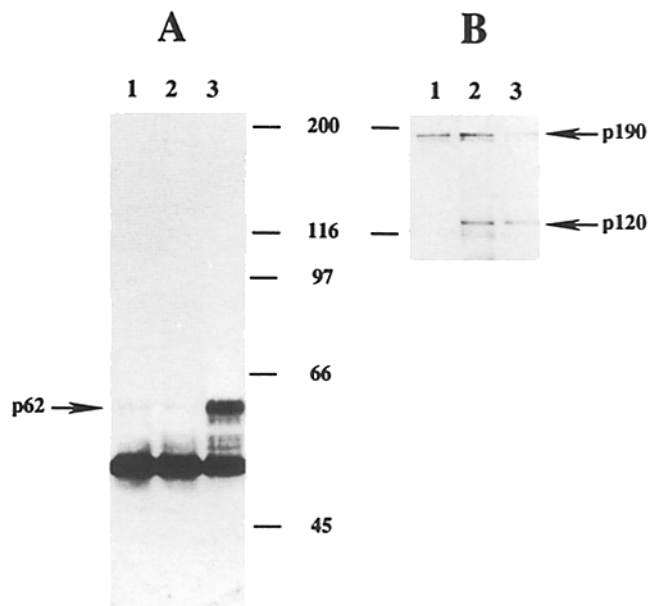
Figure 7. Only p62 is highly tyrosine phosphorylated in GAP immunoprecipitates after CD2 stimulation of Jurkat cells. (A) Jurkat cells ( 10^7 for each point) were left unstimulated (lane 1), or activated with the CD3 mAb UCHT1 for 1 min (lane 2), or the CD2 mAb pair X11+D66 for 5 min (lane 3). Cells were then lysed in a lysis buffer containing 1% digitonin and lysates immunoprecipitated with anti-GAP mAb. Immune complexes were resolved by SDS-PAGE on a 8% acrylamide gel, and Western blot analysis using antiphosphotyrosine mAb 4G10 was performed. After ECL reaction, exposure of the film was 1 min. (B) The top of the same blot after a 5-min exposure of the film.
