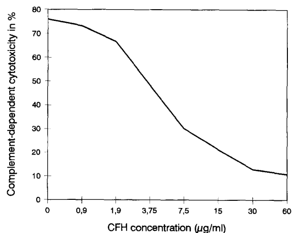
Figure 2. Effect of addition of CFH to CFH-depleted serum. The CDC decreased as increasing amounts of CFH were added. The percentages of CDC were determined as described in Materials and Methods.
