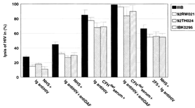
Figure 3. Lysis of cell-free HIV by human serum. Different HIV isolates (the lab strain HIV-IIIIB and three primary isolates) were incubated with NHS or serum from a patient with total CFH def in the presence of purified IgG from sera of HIV + individuals (Ig anti-HIV). In some assays, anti-DAF antibodies were added as indicated. The percentage of complement-mediated lysis was monitored by measuring free p24 in the supernatant as described in Materials and Methods.
