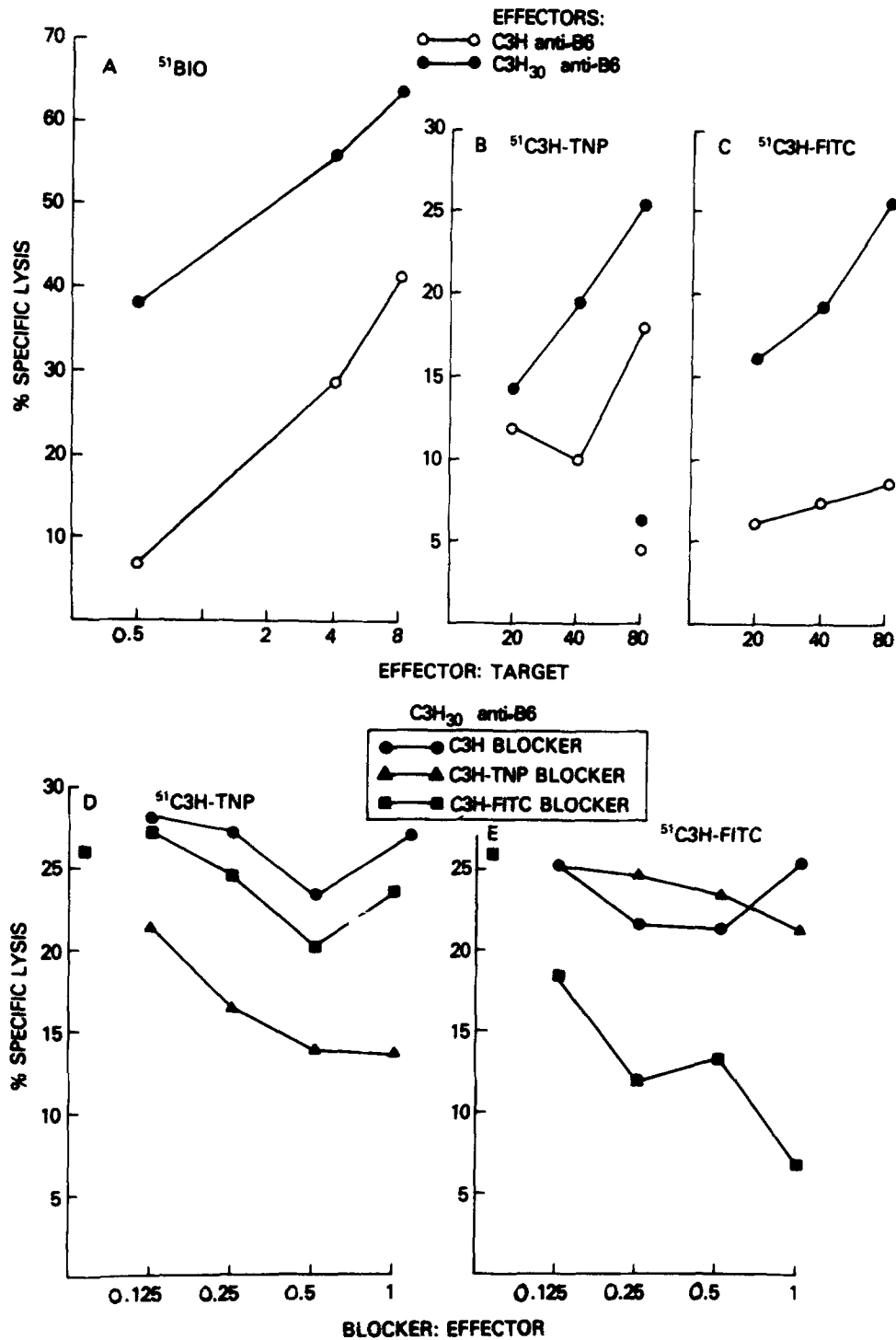
FIG. 3. Spleen cells from normal (○) or allogeneic ( H-2^b ) primed (●) C3H mice were stimulated with B6 ( H-2^b ) spleen cells and assayed on B10 ( H-2^b ) (A), C3H-TNP (B and D), and C3H-FITC (C and E) PHA-stimulated target cells (B) ○ and ● represent lysis by these effector populations on unmodified C3H target cells at 80:1. In D and E, ■ represents the lysis by primed C3H anti- H-2^b effectors on C3H-TNP and C3H-FITC at an effector target ratio of 80:1, in the absence of blocking cells. Cold target blocking populations were added at the indicated blocker effector ratio as described in Materials and Methods (D and E). C3H-anti-C3H cultures from the responding populations mediated from -5.2 to 8.1% lysis at 80:1 on C3H-TNP and C3H-FITC targets. Spontaneous release: C3H, 30.9%, C3H-TNP, 30.0%, C3H-FITC, 33.0%, B10, 22.2%.
