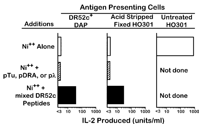
Figure 5. Peptides isolated from HO301 produced DR52c can transfer Ni^{++} presenting ability to other DR52c bearing cells. Peptides were acid stripped and purified from DR52c immunopurified from HO301 cells. An aliquot of the peptides ( 3 \times 10^8 cell equivalents) were added to either DR52c expressing DAP cells or pH3-treated fixed HO301 cells. The cells were used either before (white bar) or after (black bar) peptide exposure to present Ni^{++} (100 \mu M) to ANi-2.3 cells. As negative controls (hatched bar), peptides (pTu, pDRA, p \lambda ) known to bind well to DR52c were used (100 \mu g/ml). Presentation by untreated HO301 cells served as the positive control.
