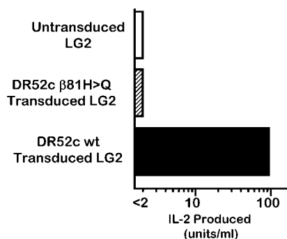
Figure 6. DR52c \beta 81His is important for ANi-2.3 recognition of DR52c presented Ni^{++} . LG2 cells were transduced with the gene for the DR52c \beta chain in which the codon for \beta His81 was changed to that for Gln. Presentation of Ni^{++} to ANi-2.3 cells by the LG2 cells transduced with the mutant \beta chain (hatched bar) was compared with that seen with untransduced LG2 cells (white bar) or LG2 cells transduced with the wild type \beta chain (black bar).
