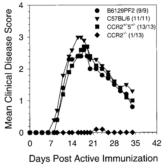
Figure 2. CCR2^{-/-} mice do not develop clinical EAE. Mice were monitored for development of clinical disease. The data are expressed as the mean clinical disease score for all mice in each group as a function of days after immunization with disease incidence indicated in parentheses. Both mean clinical disease severity and disease incidence were significantly decreased in CCR2^{-/-} animals relative to C57BL/6, B6129PF2, and CCR2^{+/-}5^{+/-} controls ( P < 0.001 ) over the entire course of the experiment. The data shown are representative of four independent experiments.
