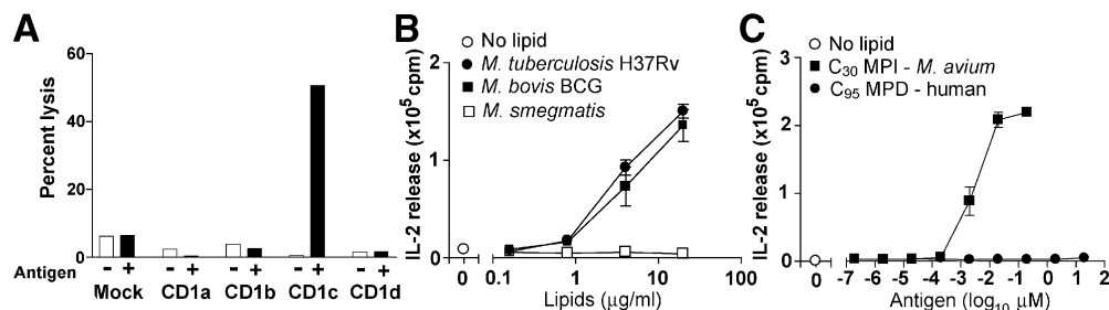
Figure 1. CD1c-restricted T cell responses for mycobacterial phospholipids. (A) Human C1R B lymphoblastoid cells transfected with the indicated CD1 genes were pulsed with 10 \mu\text{g}/\text{ml} MPI, labeled with ^{51}\text{Cr} , and lysed by the CD8-1 T cell line with an effector target ratio of 20:1. (B) CD1c-mediated IL-2 production in response to DCs treated with total lipid extracts from mycobacteria was measured using the HT-2 bioassay. (C) CD1c-mediated IL-2 release was measured in response to \text{C}_{30} MPI compounds purified from M. avium and \text{C}_{95} MPDs made from human dolichol.
